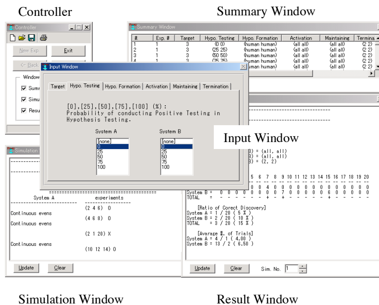
Figure 1: System's interface.
